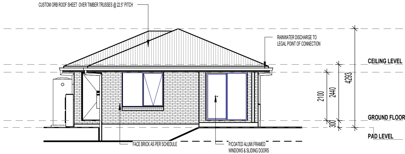
NORTHERN ELEVATION 1 : 100
