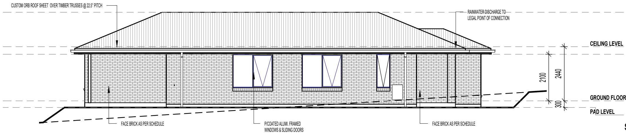
WESTERN ELEVATION 1 : 100
