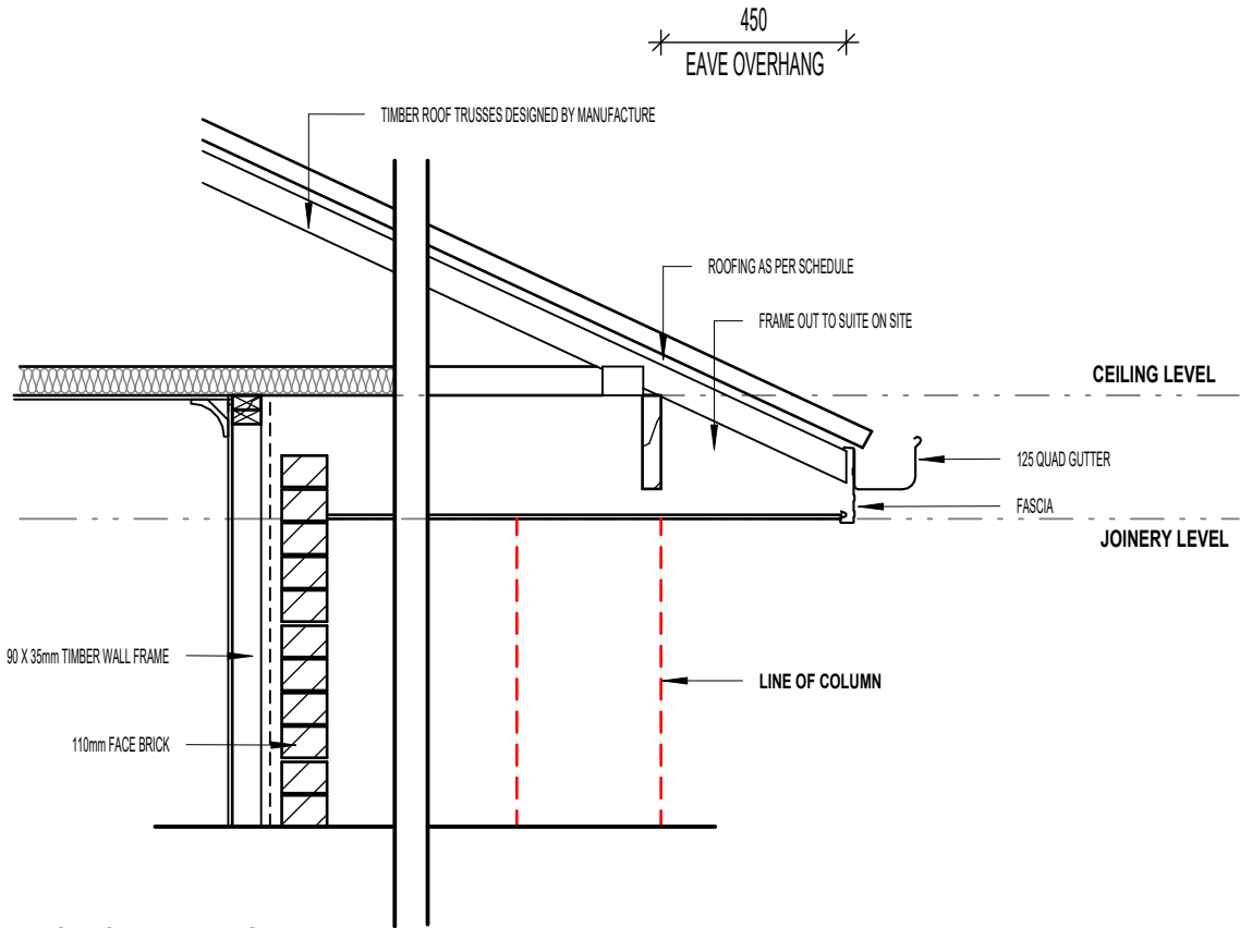
TYP. PORCH EAVES DETAIL 1 : 20
