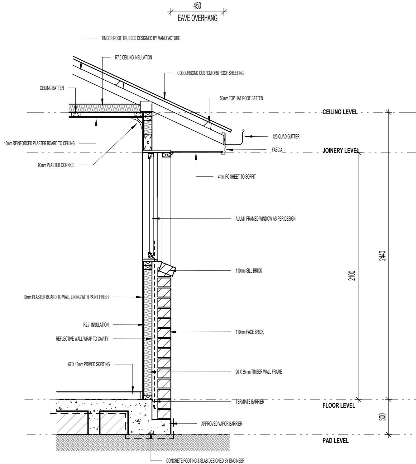
TYP. BRICK VENEER WALL DETAIL - CB ROOF 1 : 20
